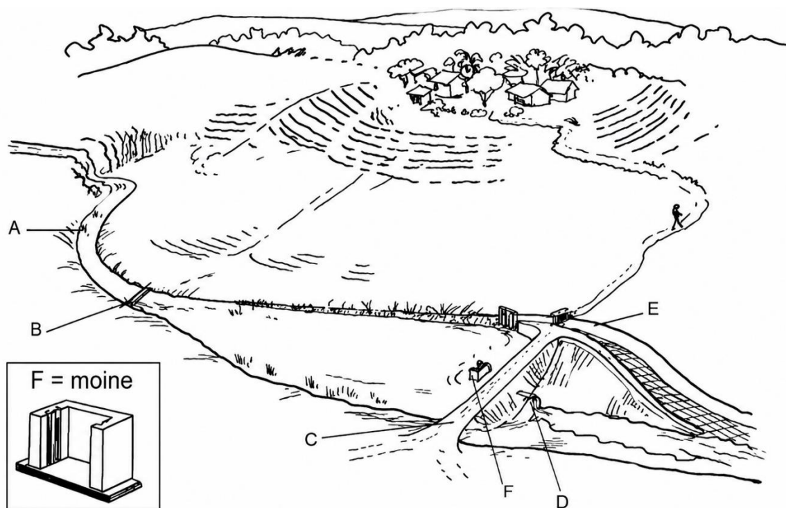
Figure 13: Etang de barrage (Source : Doc Dac_MEN))
