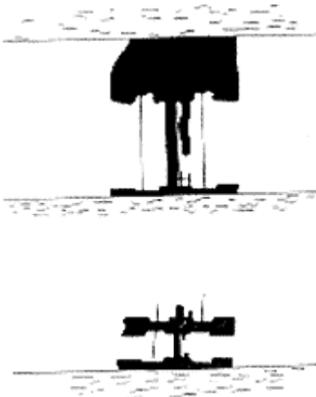
Superior mirage North Pacific Ocean
